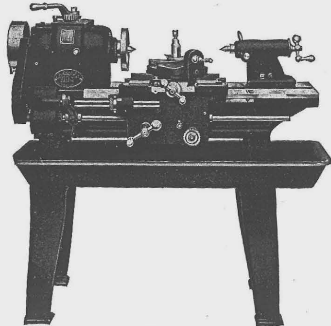
Short cut lathe—Ask us about it
